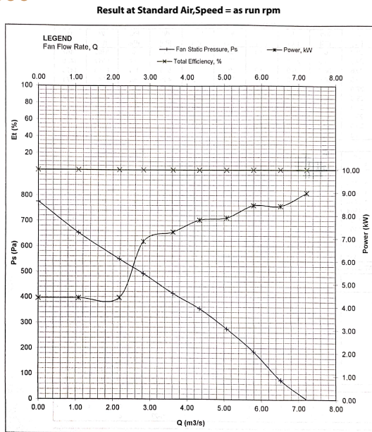
Test Method in accordance to AMCA Standard 210-07/AANSI-ASHRAE 51-07
